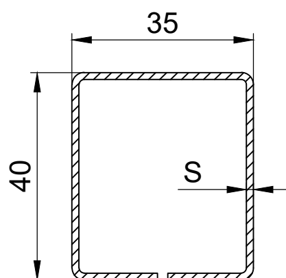
35x40x35x40
